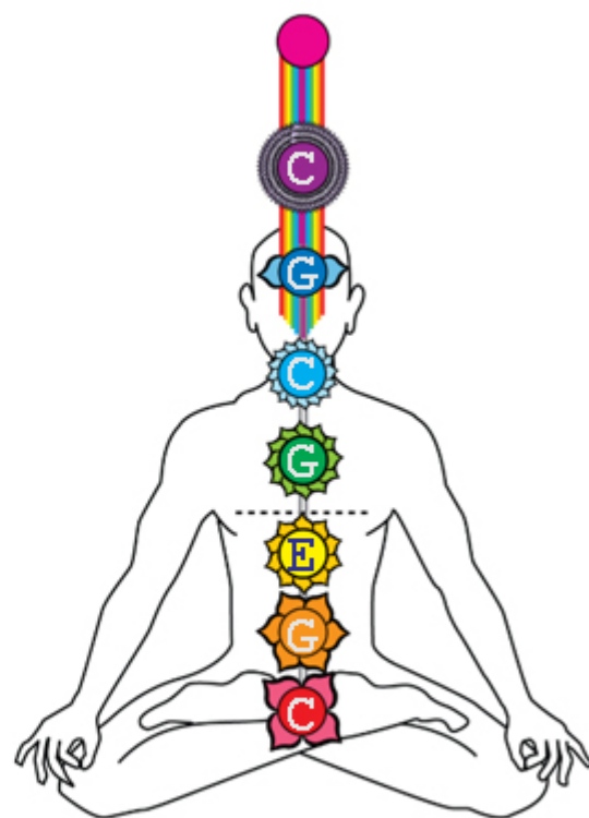
Harmonic series (4, 6, 10, 12, 16, 96)
